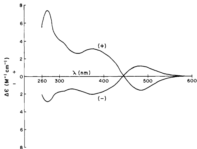
Figure 1. CD spectra of Fp[ \eta^2 -(+)-menthylvinyl ether]BF 4 and Fp[ \eta^2 -(-)-menthylvinyl ether]BF 4 taken in methylene chloride solution, on a Jobin-Yvon autodichrograph Mark 5. 22
