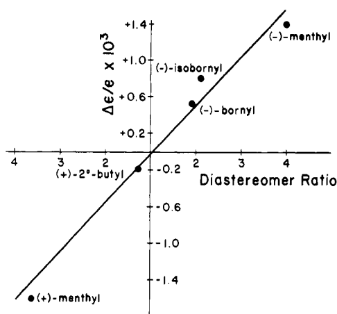
Figure 2. Correlation of normalized differential absorption \Delta\epsilon/\epsilon for a series of \text{Fp}(\eta^2\text{-vinyl ether})\text{BF}_4 complexes, derived from optically active alcohols, with the equilibrium ratio of diastereomers determined from ^{13}\text{C} spectra. Both measurements are taken at 20^\circ\text{C} .
