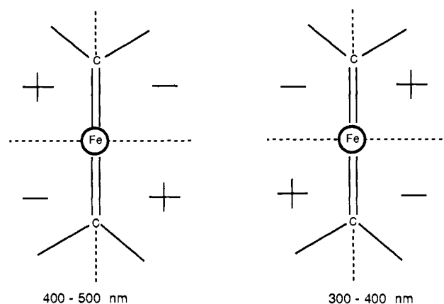
Figure 3. Quadrant rule for optically active \text{Fp}(\eta^2\text{-vinyl ether})\text{BF}_4 complexes for Cotton effect bands in the regions of 400–500 and 300–400 nm.
